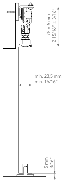
KT 80
