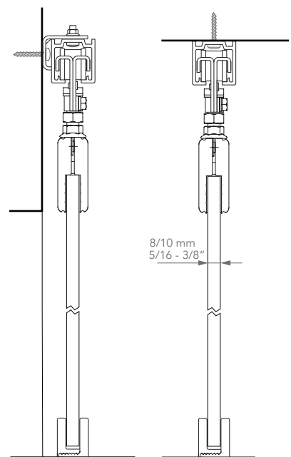
NK GLASS 80
