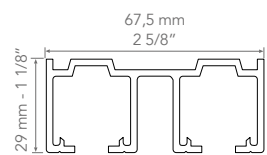
CLOS NK 60
