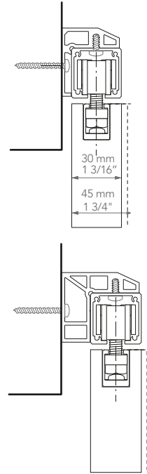
Perfil soporte pared 6 mm / Wall bracket profile 6 mm
