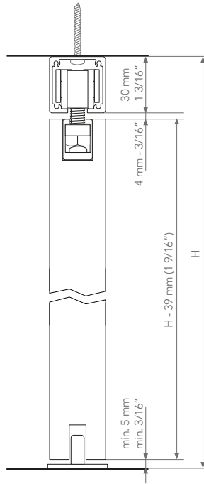
Soporte pared 6 mm / Wall bracket 6 mm
