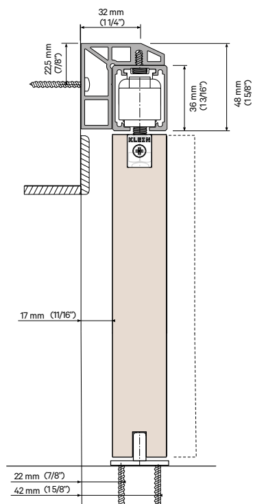
Perfil soporte pared 17 mm Wall Support Profile 17mm | Profile Support Mural 17 mm
