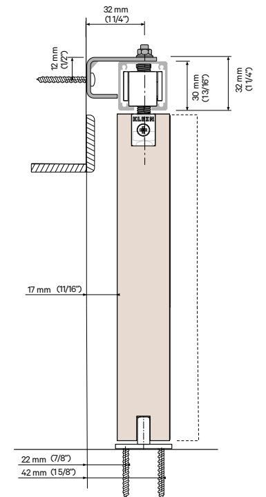
Soporte puntual pared 17 mm Point support to the wall 17mm | Support ponctuel au mur 17mm
