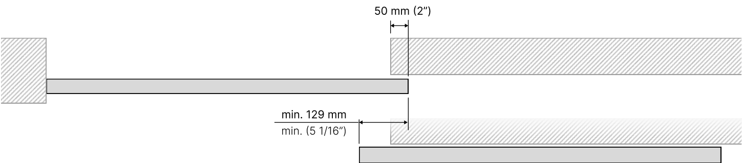
Puerta contra pared Door against the wall
