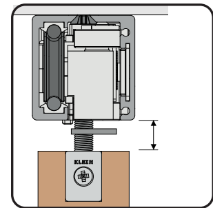
WITH LOCK 11 ± 2 mm (7/16" ± 1/16")
