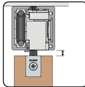
WITHOUT LOCK 6 \pm 2 \text{ mm (1/4\" } \pm 1/16\text{")}
