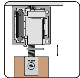
WITH LOCK 11 \pm 2 \text{ mm (7/16\" } \pm 1/16\text{")}
